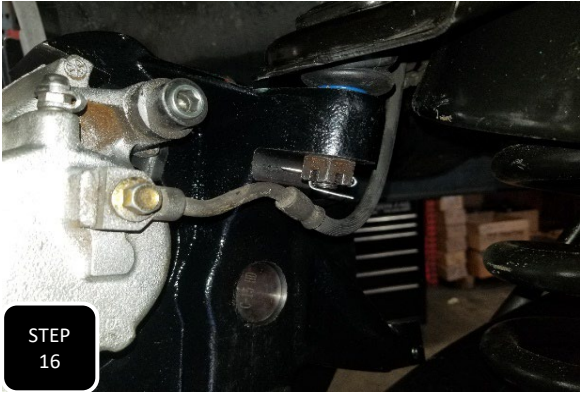
Step 16 Slide the brake caliper over the rotor and tighten down both brake caliper mounting bolts.
