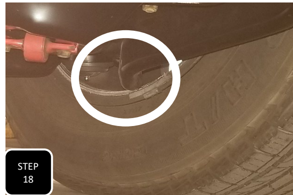
Step 18 If you plan on running smaller than 20" rims then you will need to trim the lip of the lower control arm to prevent it from contacting the wheel at full turn.
