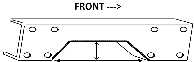
Step 5 Before being able to test fit the frame support, you will need to trim the bed rib, directly above, in order for the frame support to be able to slide over the top of the frame. Using a suitable cutting device, trim the bed rib about 1/2" up from the bottom. Trim from the end of the rib to at least the inside edge of the frame to ensure an easy install of the frame support and no contact of the two.
