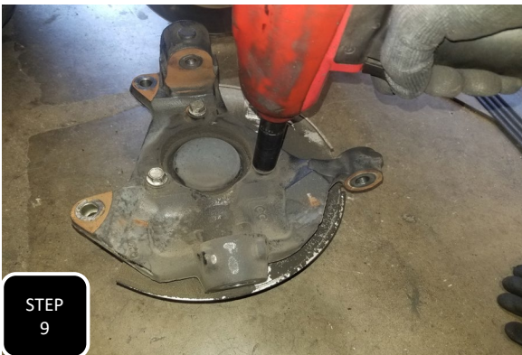
Step 9 Remove the 3 hub mounting bolts and separate the hub from the spindle.
