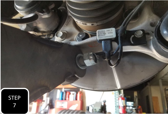
Step 7 Attach the control arm to the spindle using the factory bolt and provided M18 nut/washer then fully tighten to factory specs.
