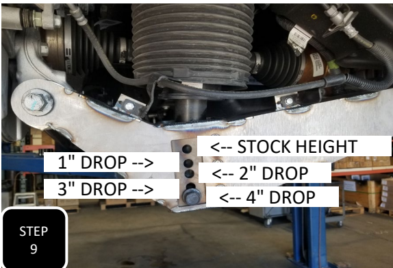
Step 9 Adjust the height of the control arm until the bottom of the strut lines up with the appropriate hole. Next, install the factory bolt and tighten to factory specs.
