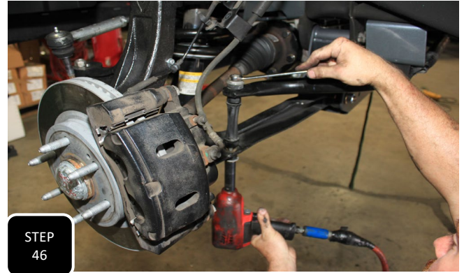
Step 46 Assemble the sway bar end links onto the truck and then tighten them up until the nut bottoms out.
