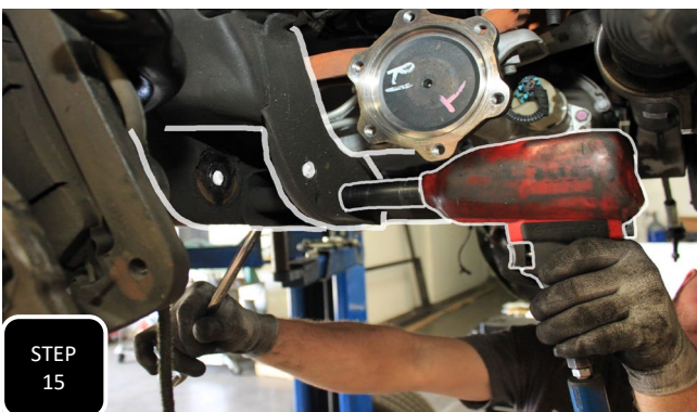
Step 15 Unbolt the 4 bolts attaching the cross member to the rearward lower control arm mount and remove the cross member.
