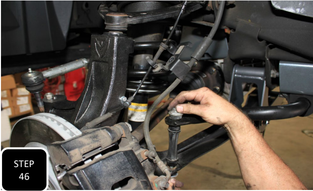
Step 46 Assemble the sway bar end links onto the truck and then tighten them up until the nut bottoms out.
