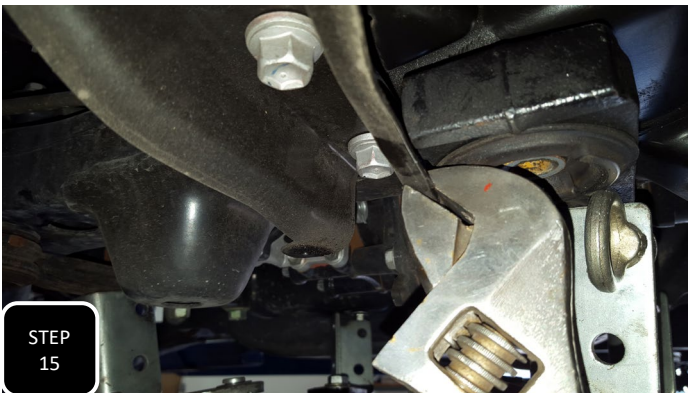
Step 15 For models with stamped steel supports, bend down the lip of the sub frame support to make way for the diff mount in its new, lower position.
