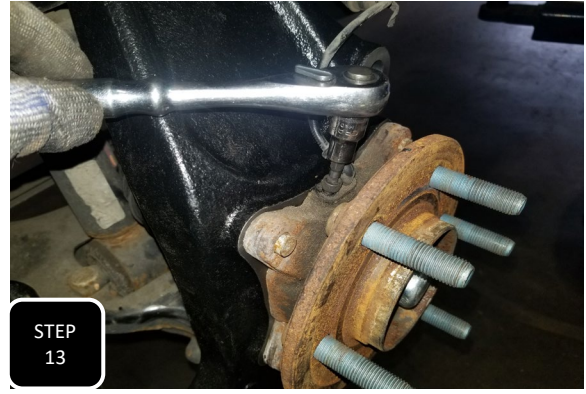
Step 13 Install the ABS sensor into the wheel bearing using the factory bolt and tighten.
