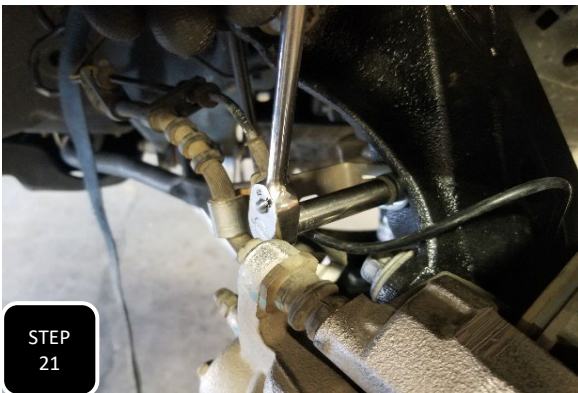
Step 21 Attach the brake/ABS line guide bracket to the side of the spindle using the factory bolt and tighten.
