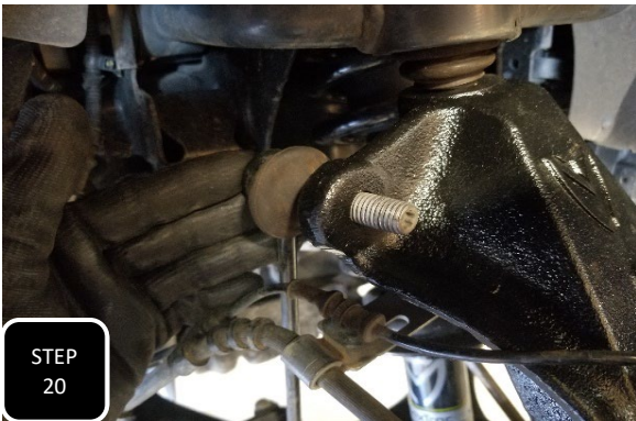
Step 20 Attach the sway bar end link to the spindle using the factory nut and tighten.
