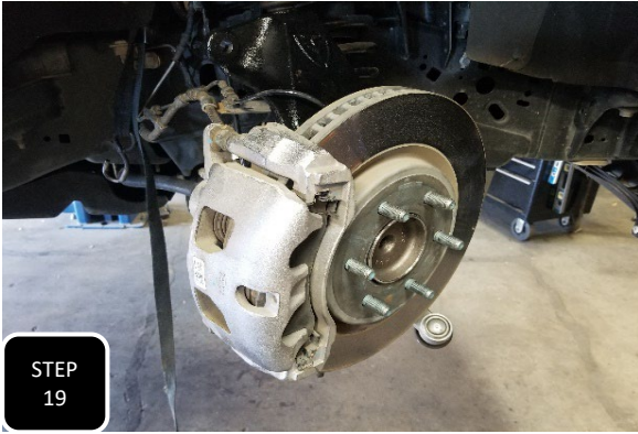
Step 19 Re-install the brake caliper using the factory bolts and tighten.
