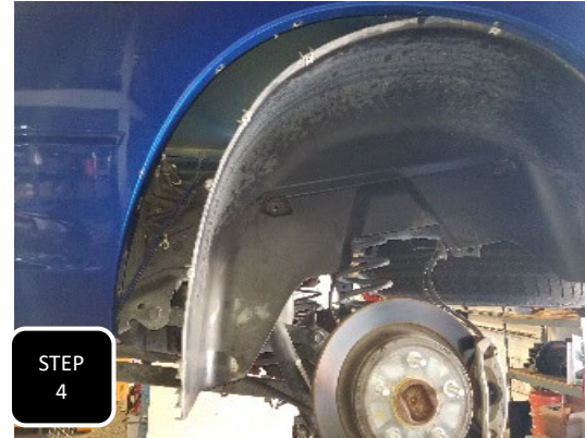
Step 4 Remove the plastic wheel liner on both sides to gain access to the upper shock mount.
