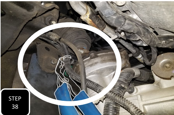
Step 38 There is a wire guide clip for the front diff electrical plug located on the frame near where the steering shaft meets the steering rack. This clip needs to be separated from the frame to allow for extra slack in the line. Next, Plug the pig tail into the diff and engage the red safety clip.
