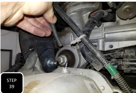
Step 39 Stretch the diff breather line down and connect it to the nurlled post on the top of the diff.
