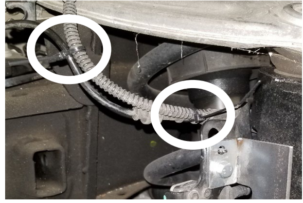
Step 7 Using the provided zip ties, attach the ABS line to the body position sensor wire.
