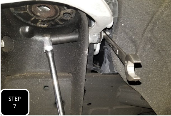
Step 7 Loosen and remove both frame mounting bolts for the upper control arm and then remove the control arm.
